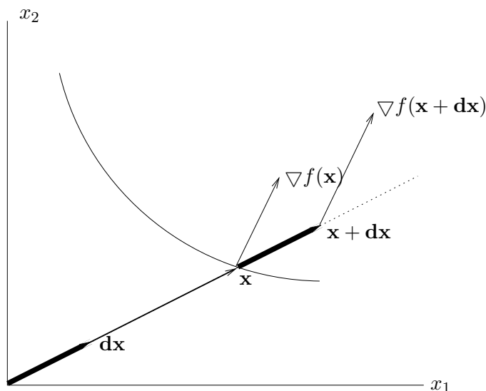
FIGURE 3. f is homothetic
