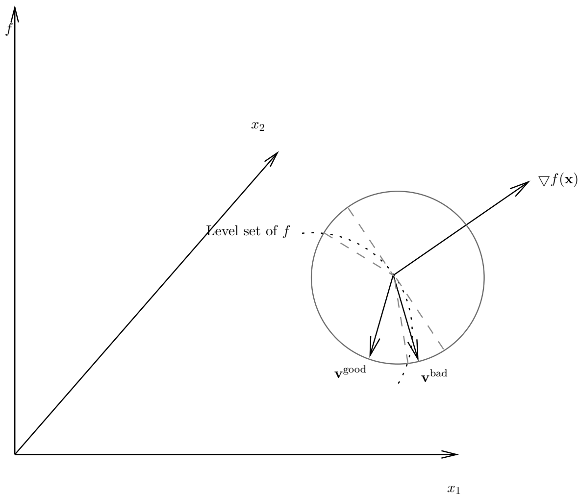
FIGURE 8. No \epsilon > 0 works for all directions
