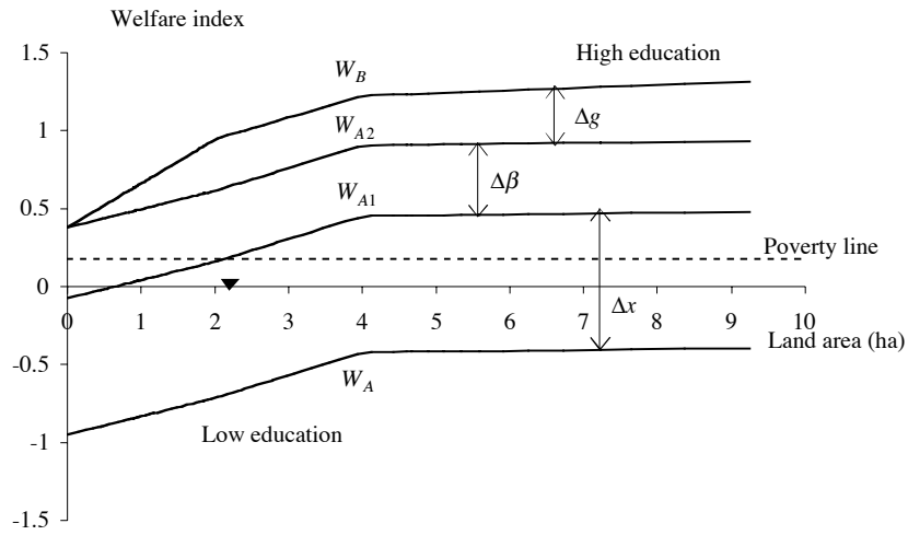
Figure 7: Welfare as a function of land assets: Role of complementary asset
