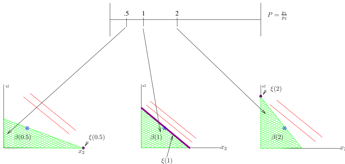
FIGURE 5. The demand correspondence is u.h.c
