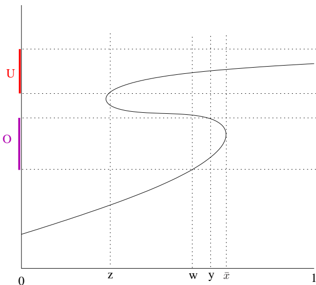
FIGURE 4. \xi : [0, 1] \rightarrow \mathbb{R}
